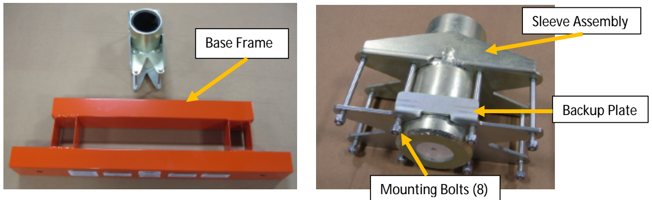
Figure 7, Disassembled Base Frame / Sleeve (Pro-3 HD is Similar)
