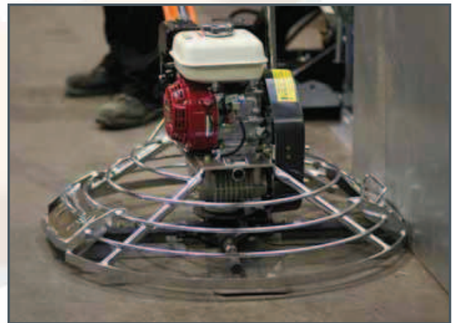
Sliding guard rail for wall trowelling
